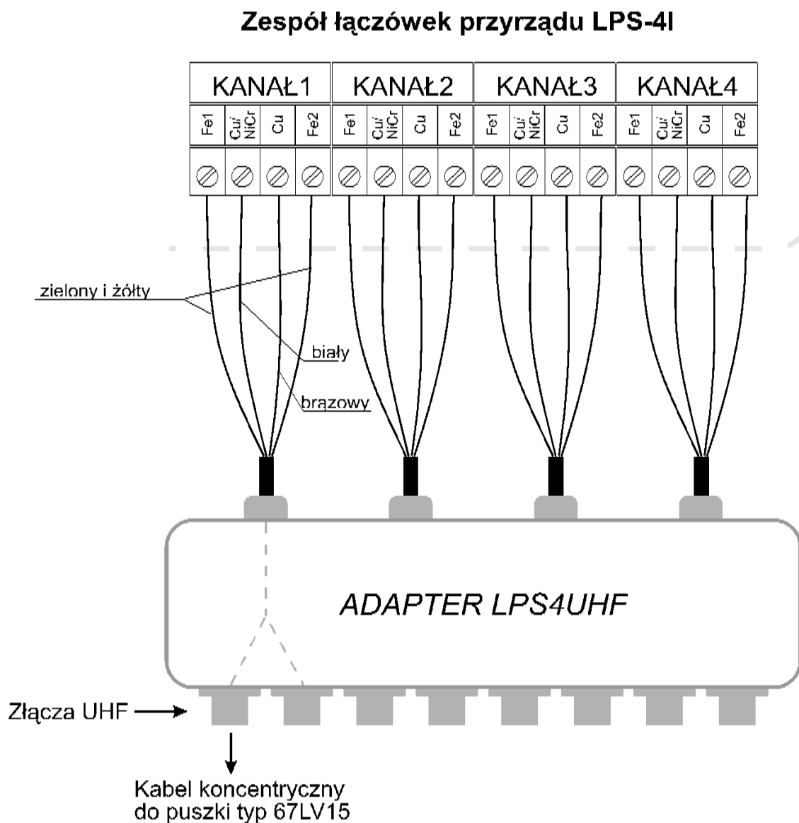
General arrangement drawing showing the method of connecting an LPS-4i meter and an LPS4UHF adapter.
